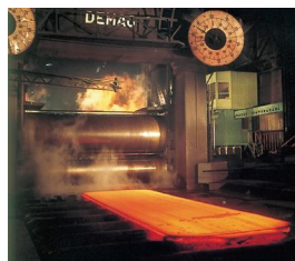
4重可逆式広巾厚板圧延機 4-High Plate Mill
